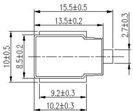
DO-218AB
