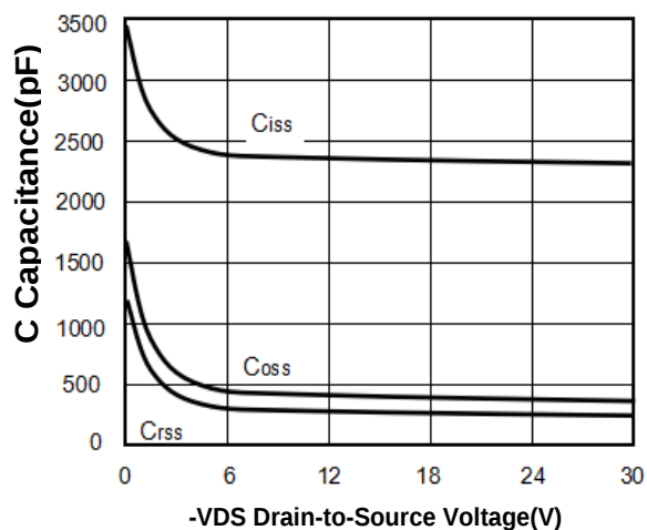
Figure5. Capacitance
