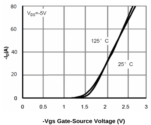
Figure4. Transfer Characteristics
