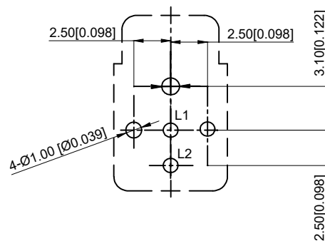
PCB.Welding diagram PCB.焊接图
