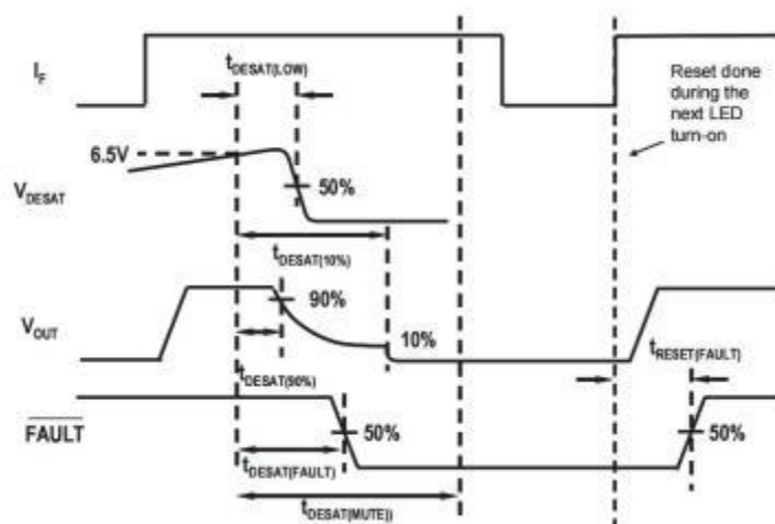
Figure 36. Fault Timing diagram
