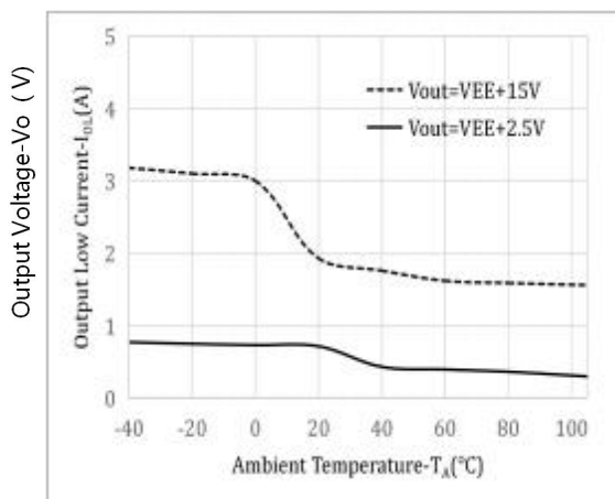
Fig.3 Output Low Current vs. Ambient Temperature
