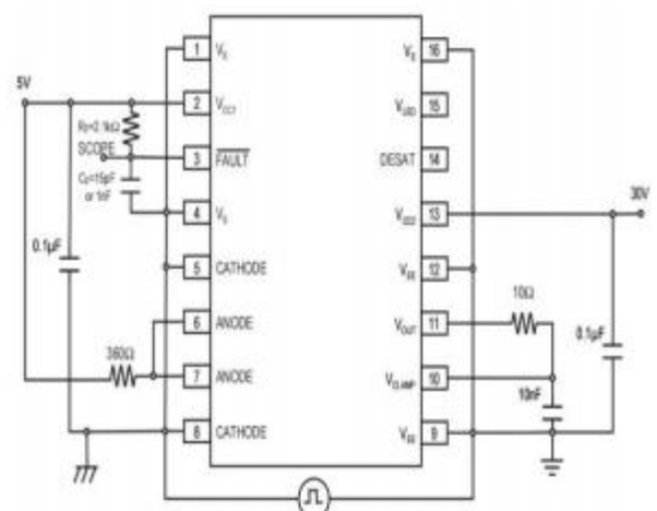
Fig 32. CMR Test Circuit LED2 on
