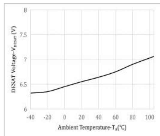
Fig.12 DESAT threshold vs. Ambient Temperature
