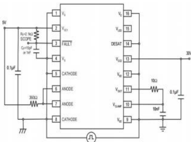
Fig 31. CMR Test Circuit LED2 off
