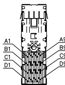
PIN NUMBERING
