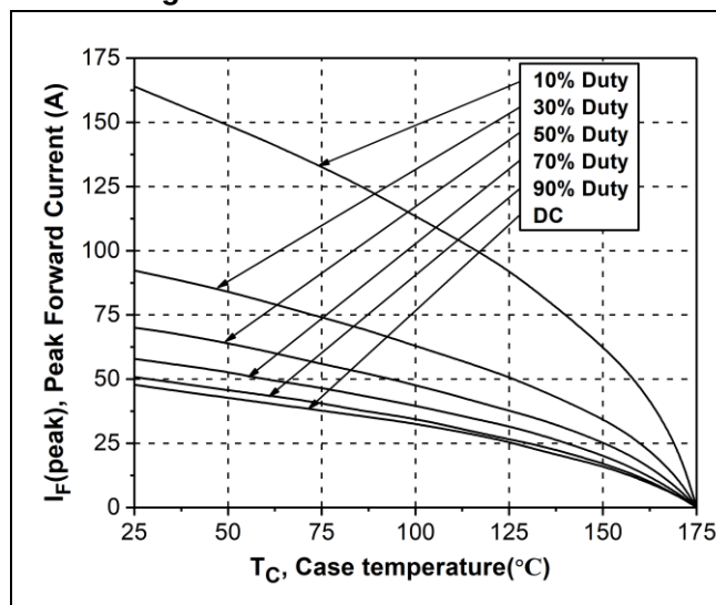
Figure 3. Current Derating
