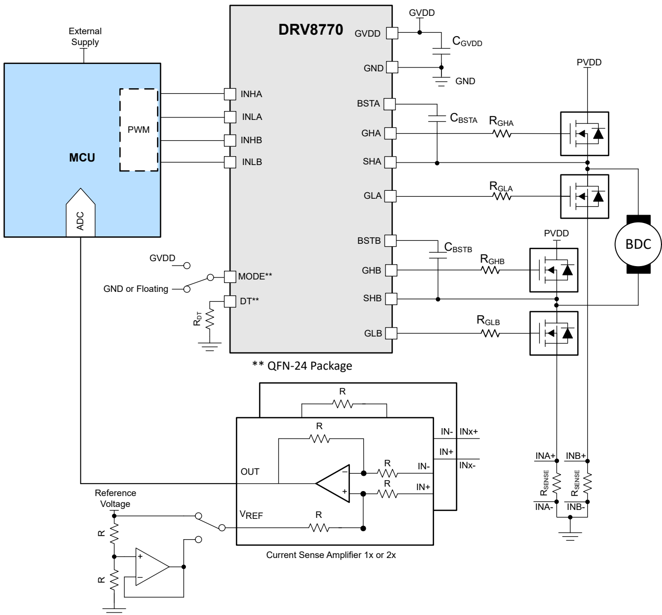
图 8-1. Application Schematic
