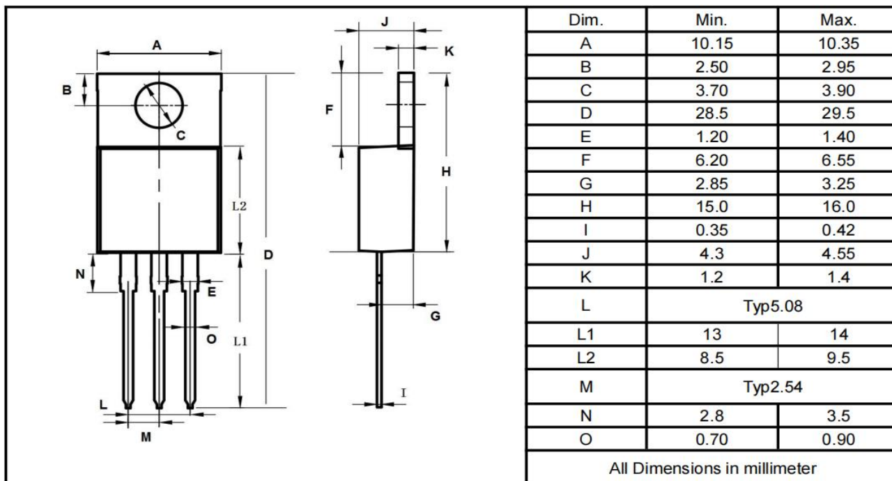
TO-220AB
