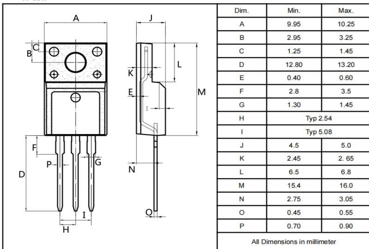
TO-220F
