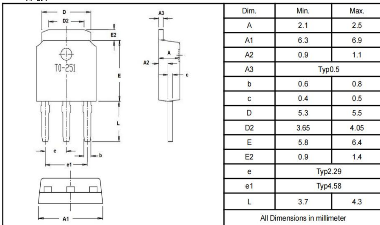
T0-251
