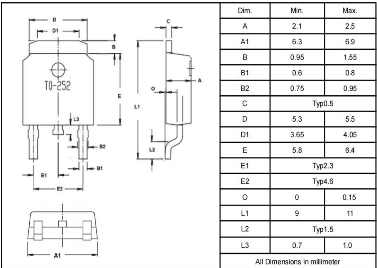
TO-252
