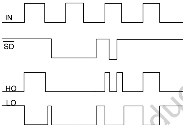
Figure 6-1 IRS2104 SInput and output timing waveform
