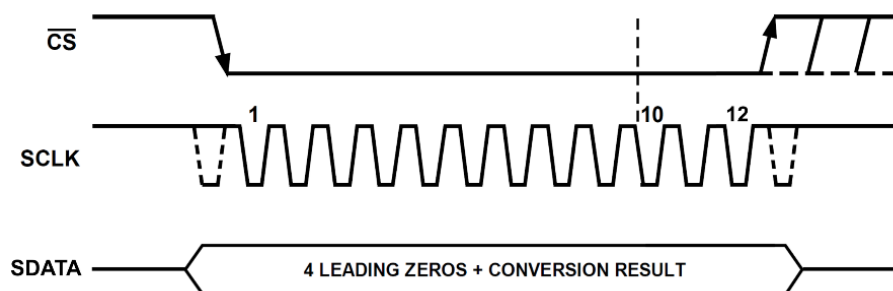
Figure 4. Timing Diagram
