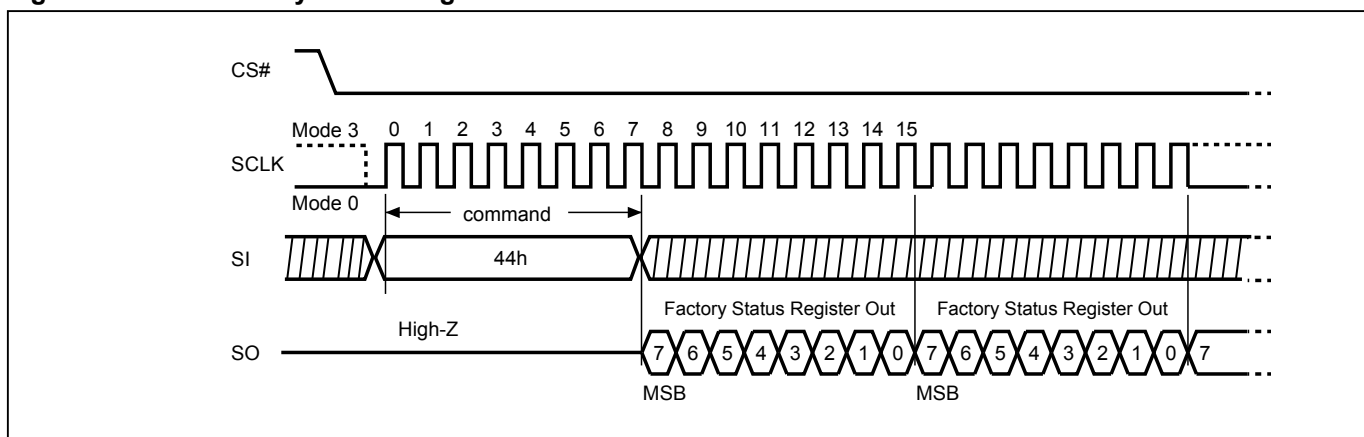
Figure 45. Read Factory Status Register
