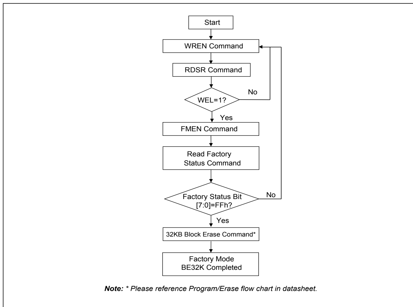
Figure 42. Factory Mode 32KB Block Erase Flow
