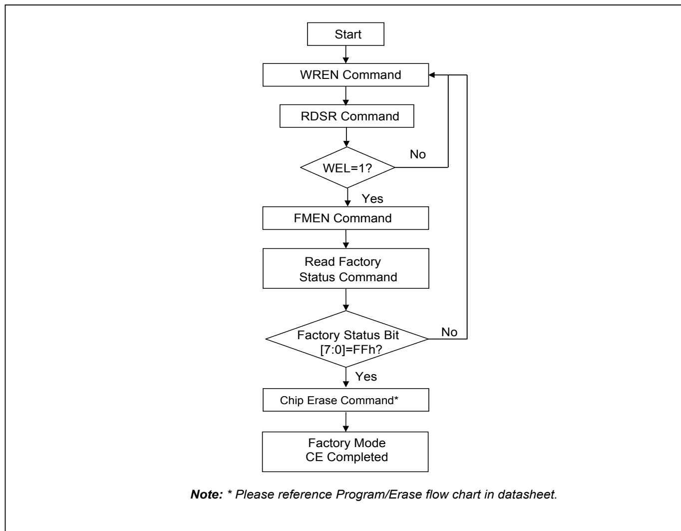
Figure 44. Factory Mode Chip Erase Flow
