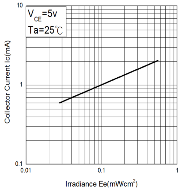
Fig.2 Collector Current Irradiance
