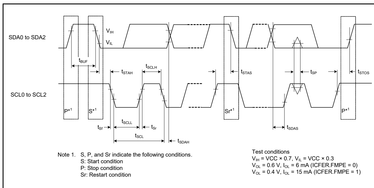
Figure 2.72 IIC Bus Interface Input/Output Timing and Simple IIC Bus Interface Input/Output Timing
