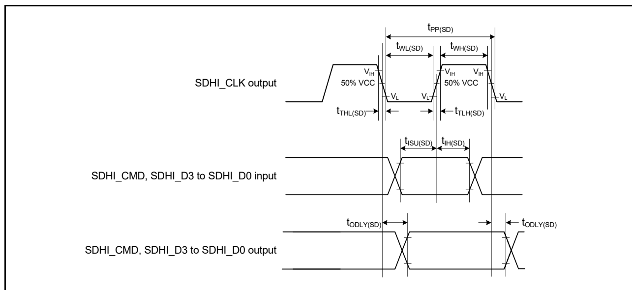
Figure 2.98 SD Host Interface Input/Output Signal Timing
