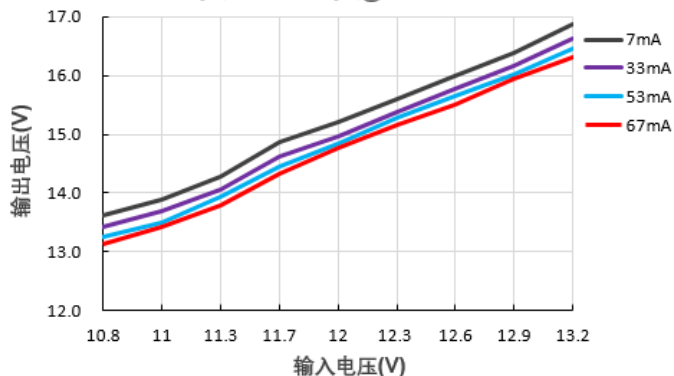
输出电压Vs输入电压@B1215S-1WR3
