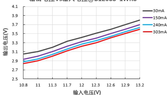
输出电压Vs输入电压@B1203S-1WR3
