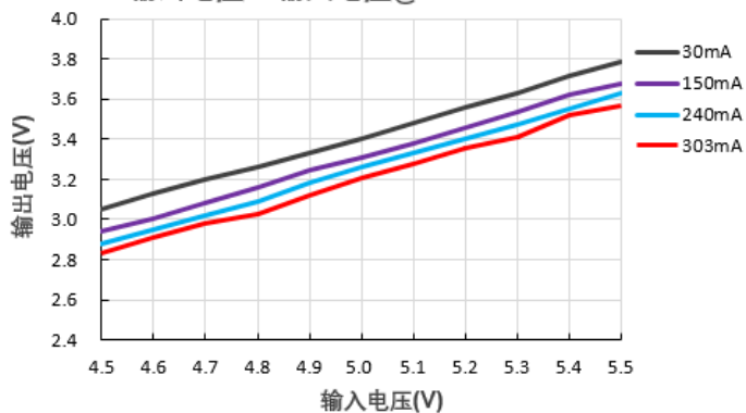
输出电压Vs输入电压@B0503S-1WR3
