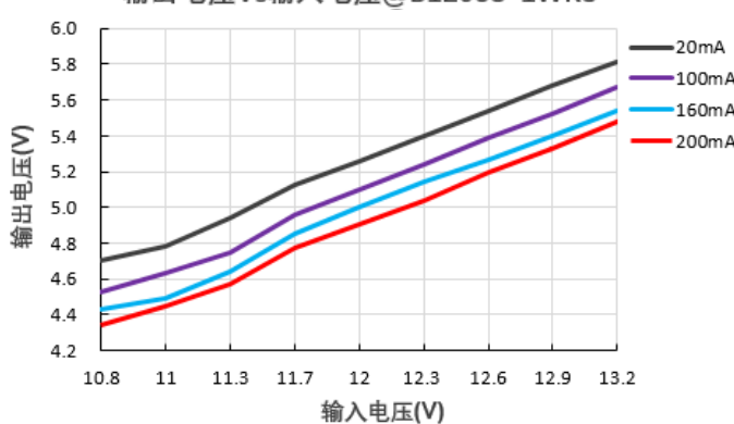
输出电压Vs输入电压@B1205S-1WR3
