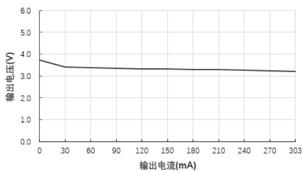
输出电压Vs输出电流(Vin=12V)@B1203S-1WR3
