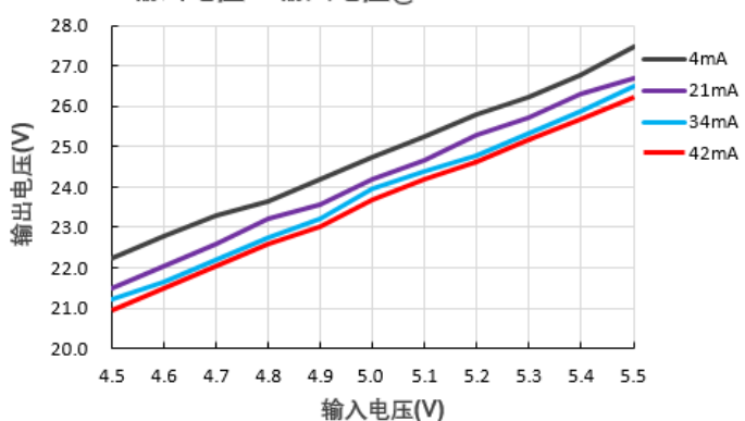
输出电压Vs输入电压@B0524S-1WR3
