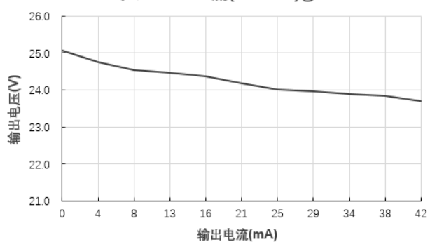
输出电压Vs输出电流(Vin=5V)@B0524S-1WR3
