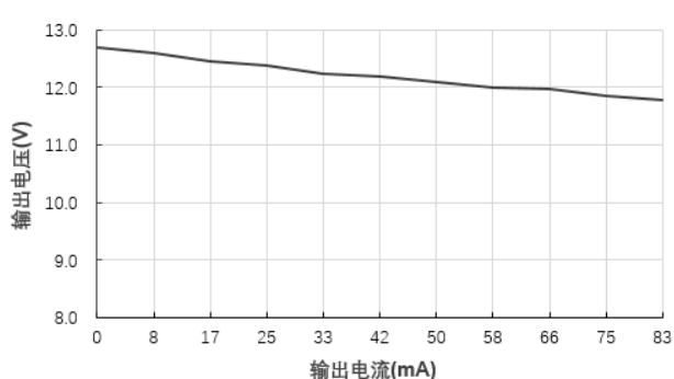
输出电压Vs输出电流(Vin=5V)@B0512S-1WR3
