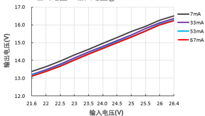
输出电压Vs输入电压@B2415S-1WR3
