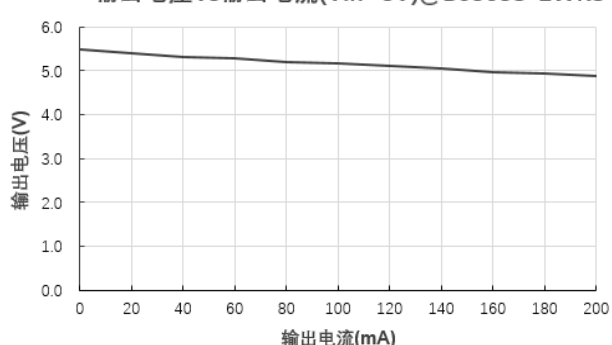
输出电压Vs输出电流(Vin=5V)@B0505S-1WR3
