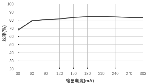
效率Vs输出电流(Vin=12V)@B1203S-1WR3
