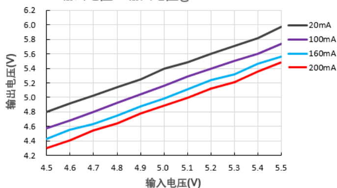
输出电压Vs输入电压@B0505S-1WR3
