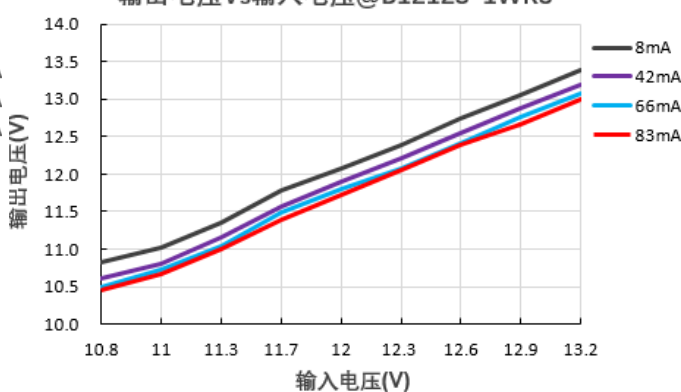
输出电压Vs输入电压@B1212S-1WR3
