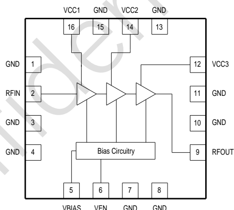
Figure 2. GDM3528 Function Block Diagram
