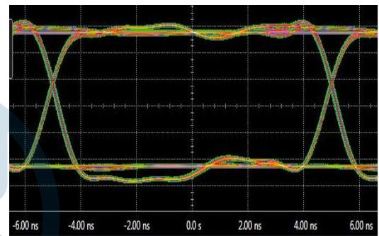
Figure 10. \pi 110E3x Eye Diagram
