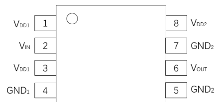
Figure 3. \pi 110E3x Pin Configuration
