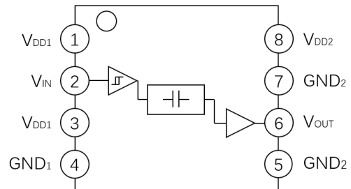
Figure 1. \pi 110E3x functional Block Diagram
