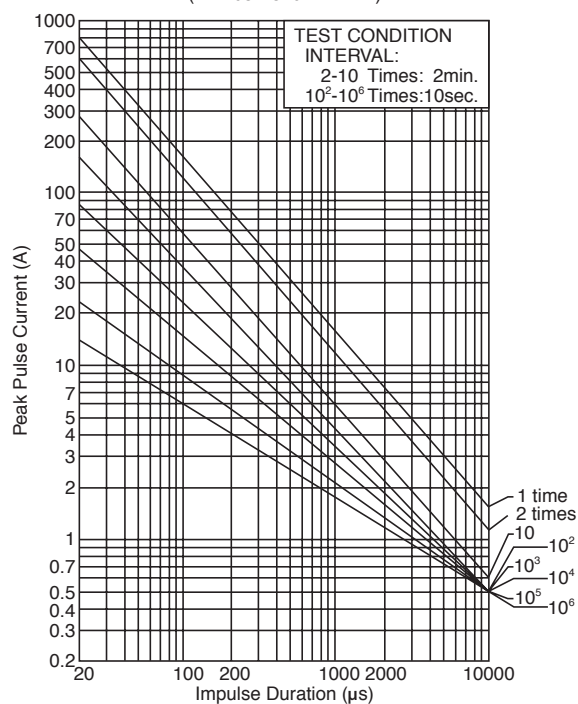
PULSE LIFE TIME RATINGS (TND05V-820K~471K)
