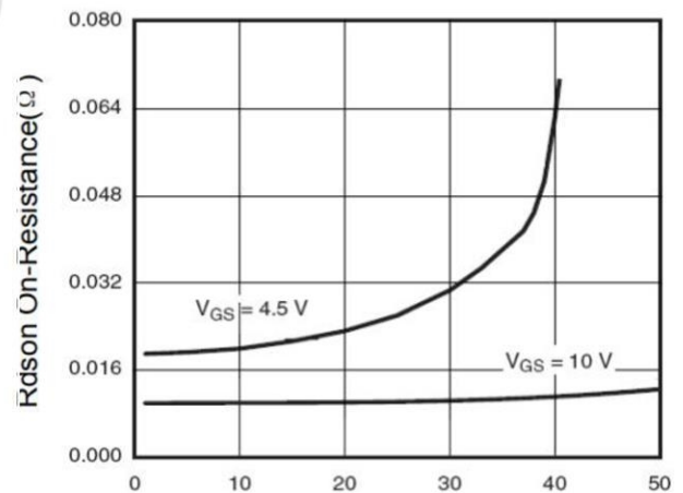
Figure 6 Drain-Source On-Resistance
