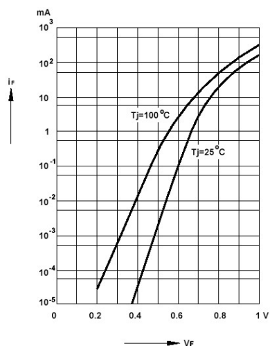
Forward characteristics
