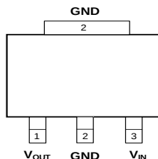
SOT89-3L(P) Top View
