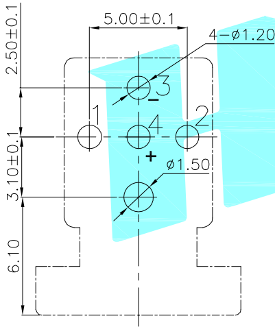
PCBLayout(pattern Side)
