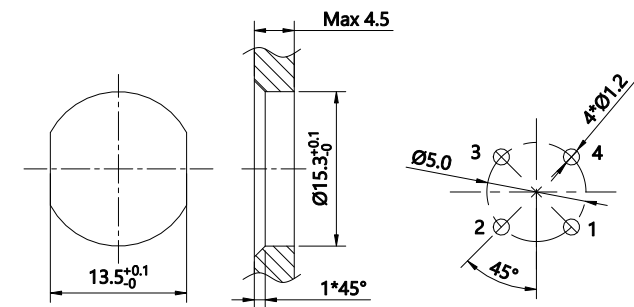
Recommended panel cut-out and PCB layout
