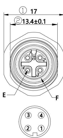
PIN View from front
