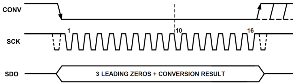
Figure 4. Timing Diagram
