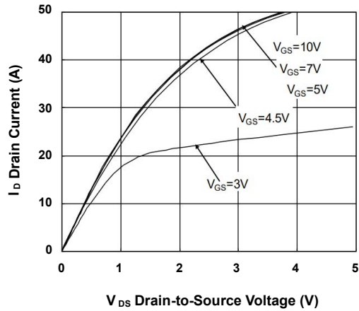
FIG.1-Typical Output Characteristics
