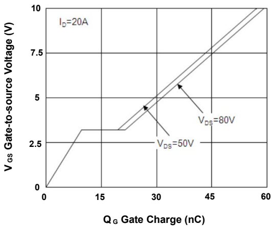
FIG.7-Gate Charge Characteristics
