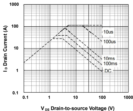
FIG.5-Safe Operating Area
