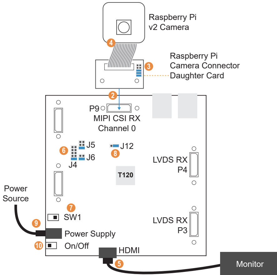
Figure 11: Hardware Setup
