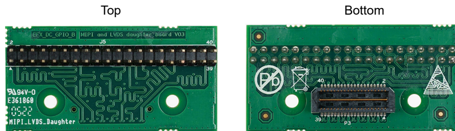
Figure 4: MIPI and LVDS Expansion Daughter Card
