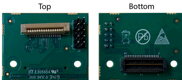
Figure 5: Raspberry Pi Camera Connector Daughter Card
