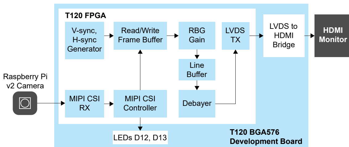
Figure 9: Debayer Filter Design Block Diagram
