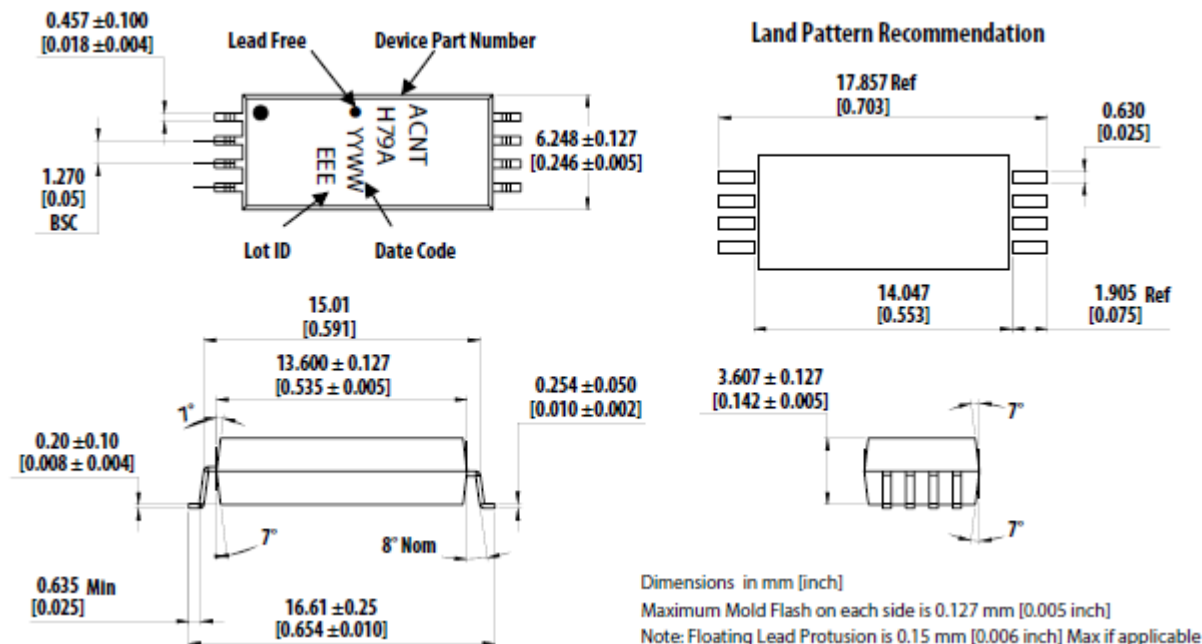
Figure 2 ACNT-H79B, ACNT-H79A, ACNT-H790 Stretched SO-8 Package
