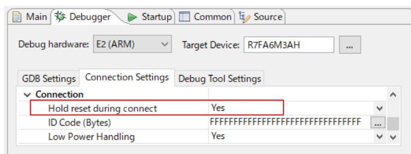
Figure 3.4 Setting of [Hold reset during connect]
