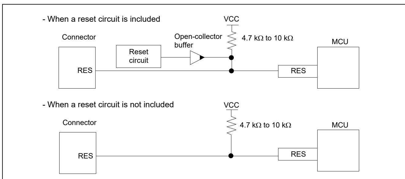
Figure 2.7 Connection of the RES Pin
