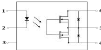
Pin Configuration
