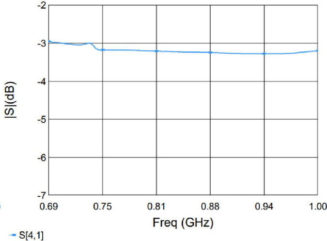
Figure 4. MHC09X03 Transmission
