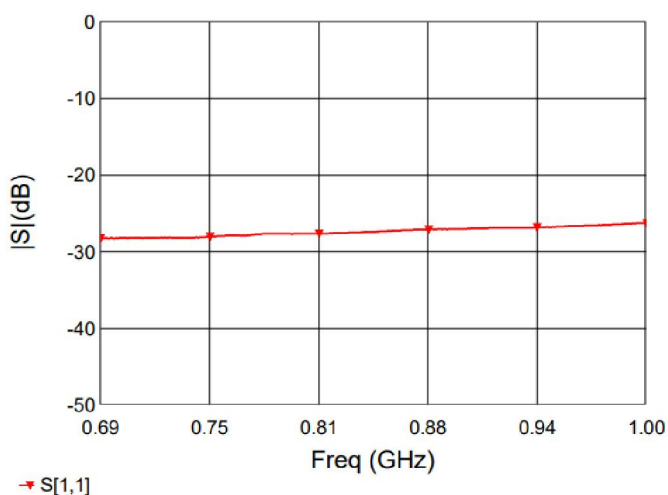
Figure 5. MHC09X03 Return Loss (S11)
