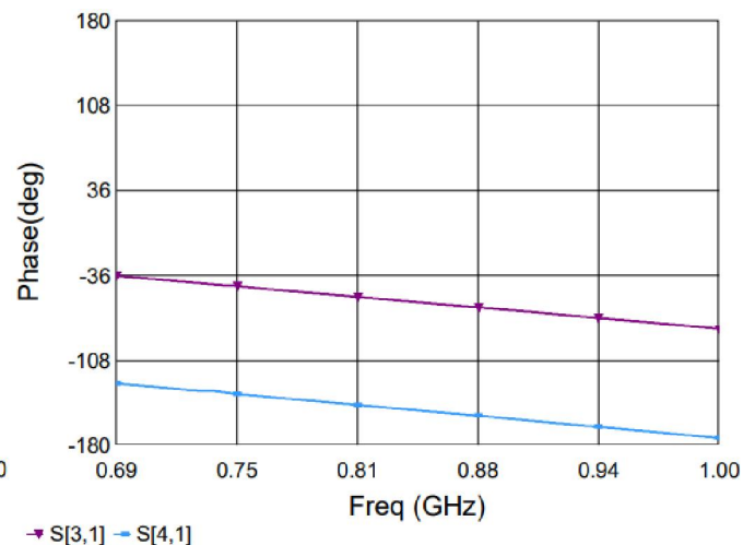
Figure 8. MHC09X03 Phase
