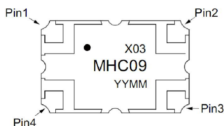
Figure 1. MHC09X03 (Top View)
