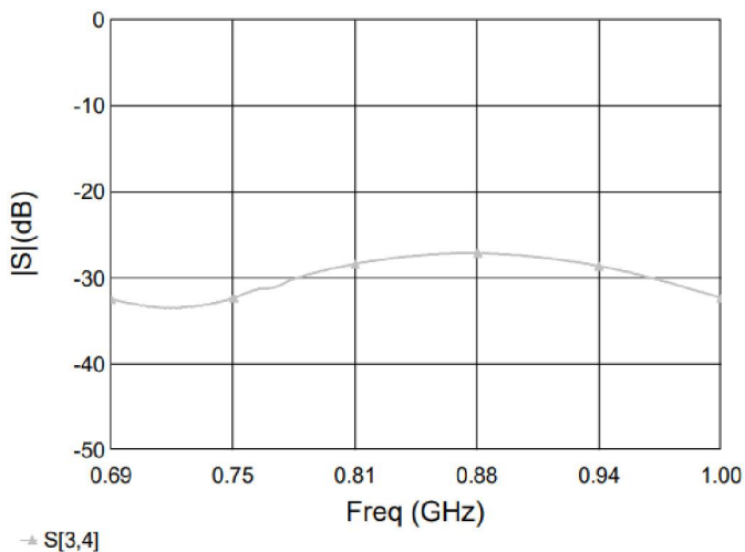
Figure 7. MHC09X03 Isolation
