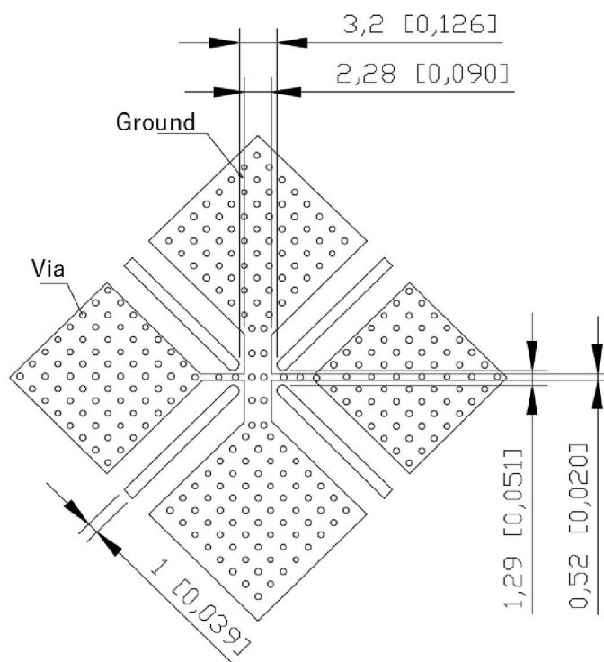
Figure 9. Recommended PCB Layout
