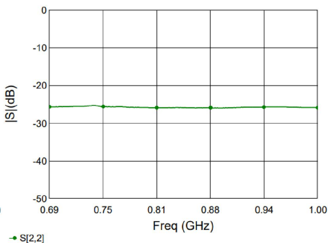
Figure 6. MHC09X03 Return Loss (S22)
