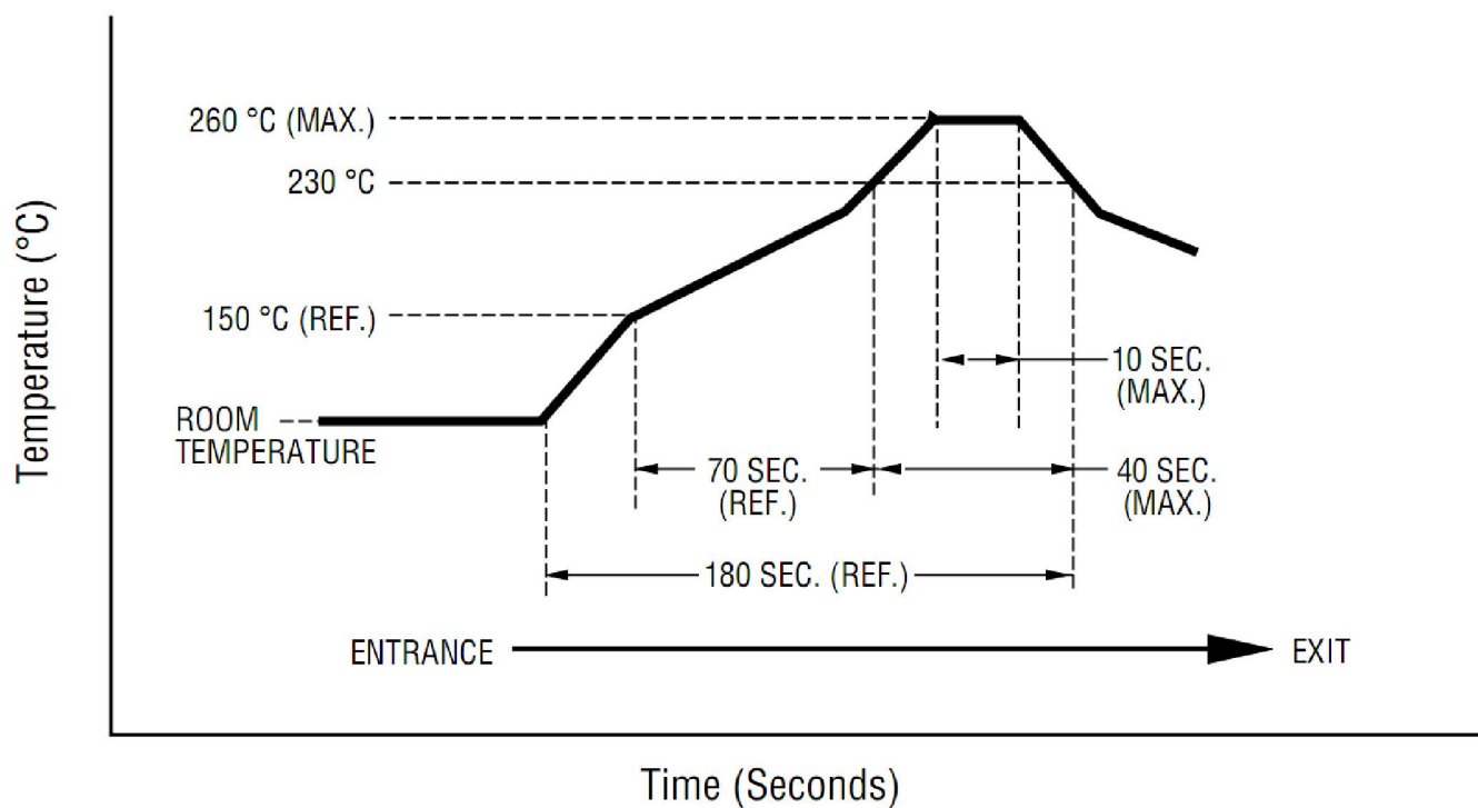
Figure 10. MHC09X03 Thermal Reflow Profile
