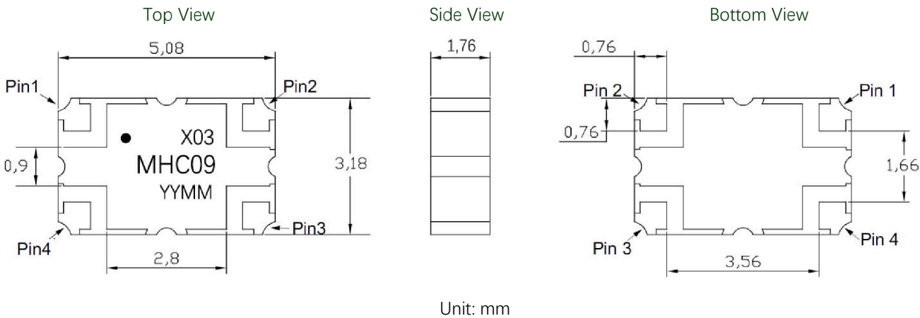
Figure 2. MHC09X03 Outline Drawing
