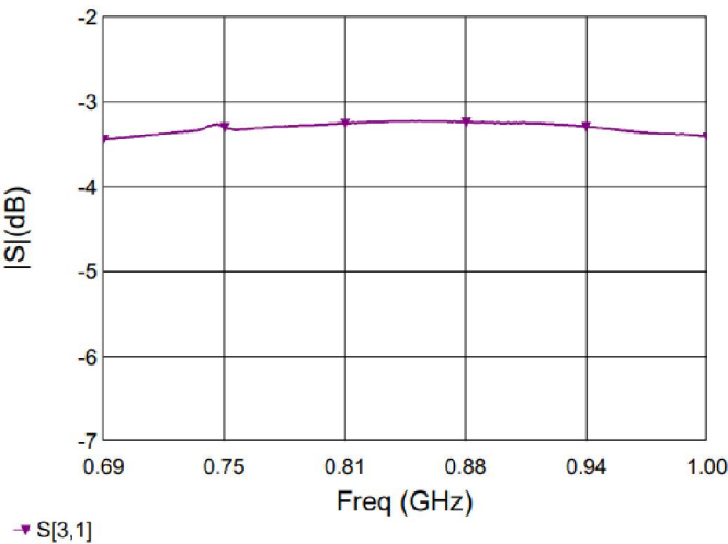
Figure 3. MHC09X03 Coupling
