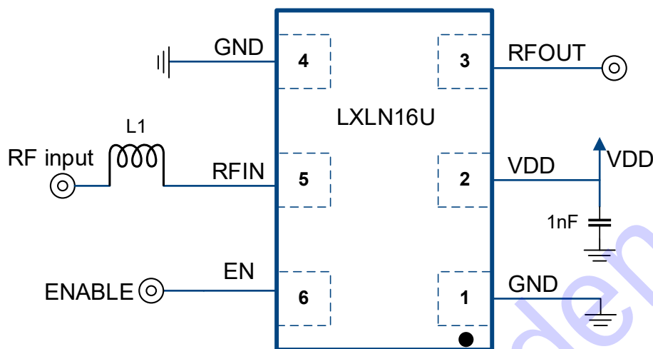
Figure 1 LXLN16U Application circuit
