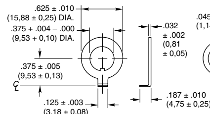
Non-Turn Washer
