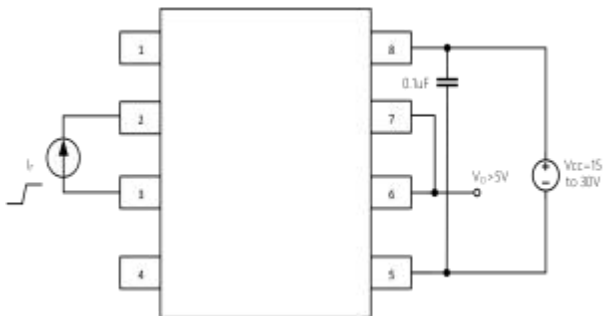
Figure.16 I_{FH} Test Circuit
