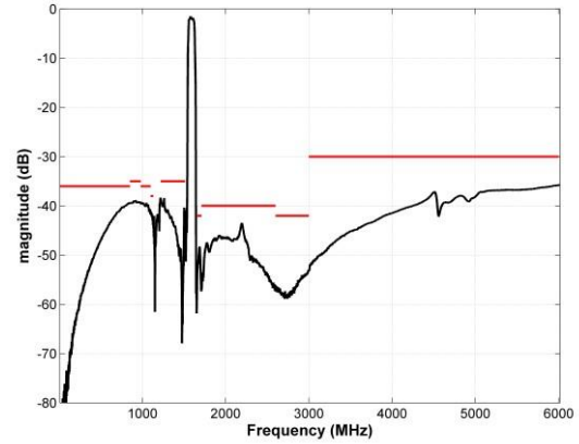
Wideband Response
