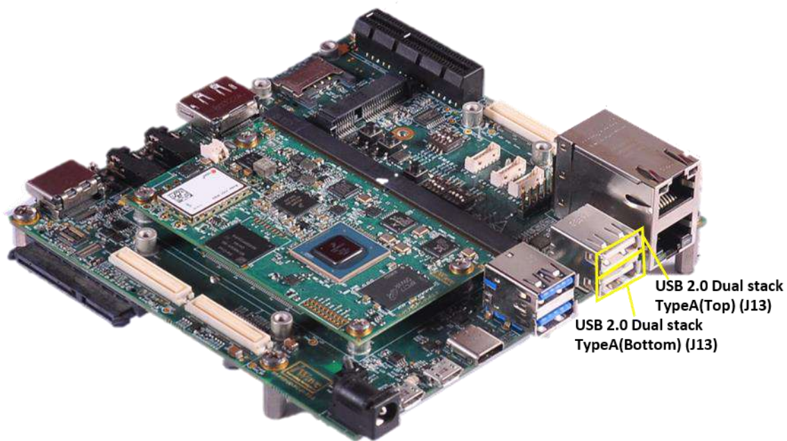
Figure 11: USB2.0 Host Port
