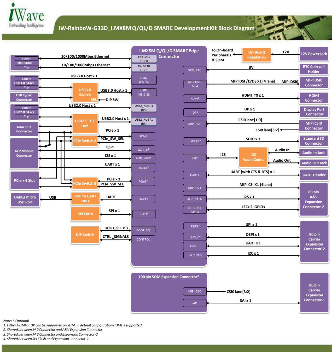
Figure 1: i.MX8M Q/QL/D SMARC Development Platform Block Diagram
