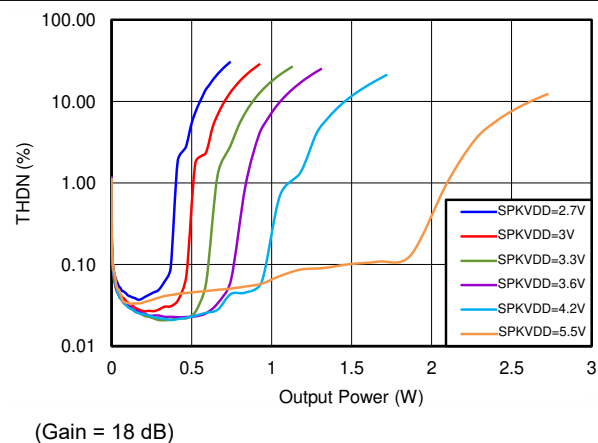
图 9-3. Total Harmonic Distortion + Noise vs 4- \Omega Speaker Power
