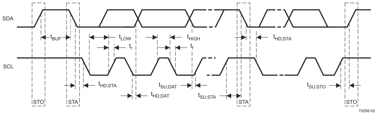
图 6-5. I²C Interface Timing
