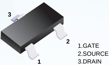
Simplified outline(SOT-23)
