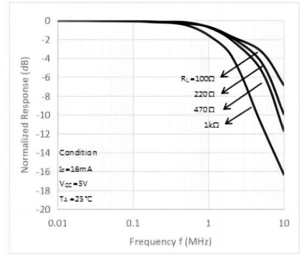
Fig.8 Frequency Response
