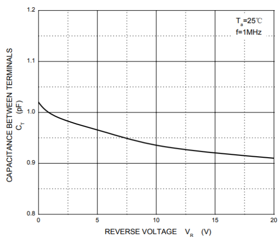
Capacitance Characteristics
