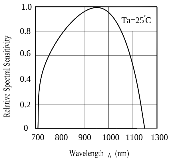
Fig.1 Spectral Sensitivity
