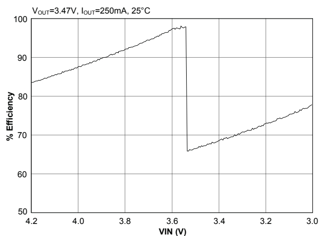
Efficiency — 250mA Spotlight
