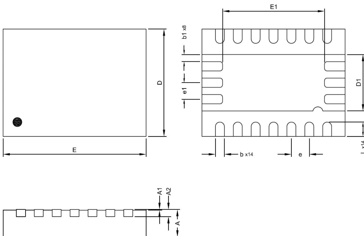
TDFN3X4-14 Package
