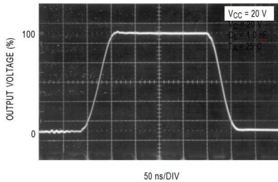
Figure 18. Bottom Drive Output Waveform
