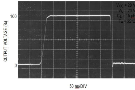
Figure 19. Bottom Drive Output Waveform
