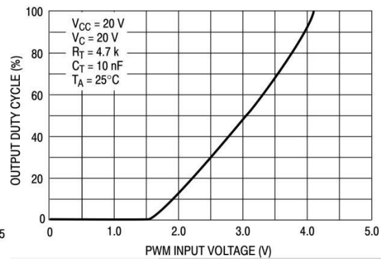
Figure 13. Output Duty Cycle versus PWM Input Voltage
