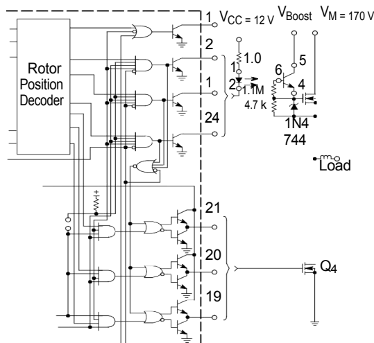
Series gate resistor R_g will dampen any high frequency oscillations caused by the MOSFET input capacitance and any series wiring inductance in the gate-source circuit. Diode D is required if the negative current into the Bottom Drive Outputs exceeds 50 mA.
