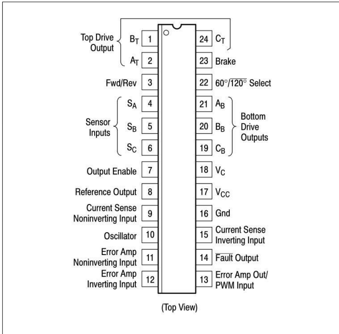
Figure 1 . PIN CONNECTIONS
