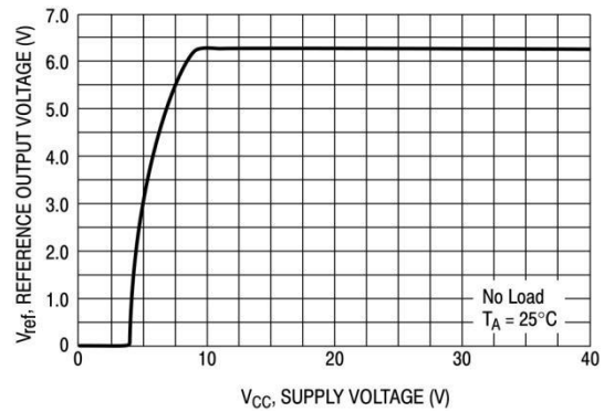
Figure 11. Reference Output Voltage versus Supply Voltage
