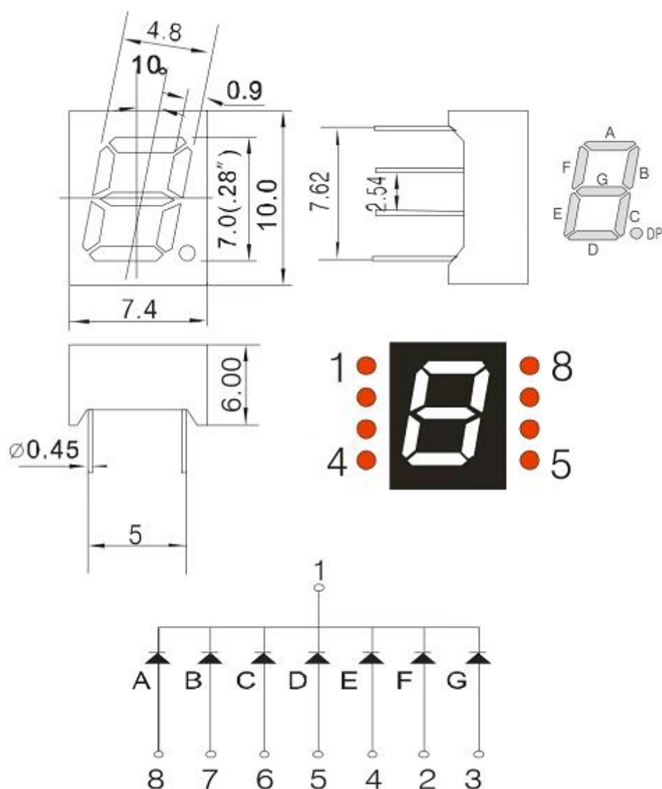
Figure Size & Circuit Principle Diagram : 7.4mm×10mm×6.0mm
