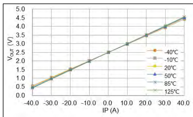
V_{out} vs. I_P
