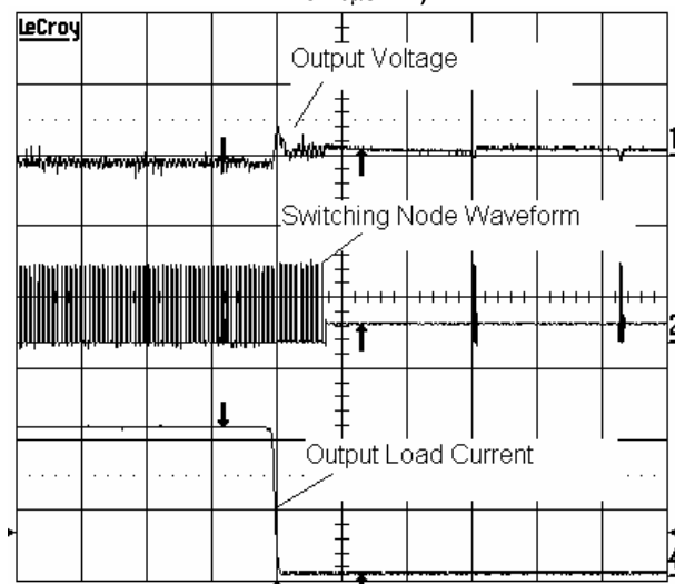
Load Transient Test ( V_{IN}=5V , V_{OUT}=1.2V , I_{OUT}=1A to 0A , PSAVE Mode Enabled, L_{OUT}=1\mu H , C_{OUT}=2 \times 22\mu F , Channel 1: 50mV/Div, Channel 2: 5V/Div, Channel 4: 0.5A/Div, Time: 20μs/Div)
