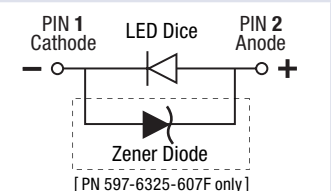
Schematic
