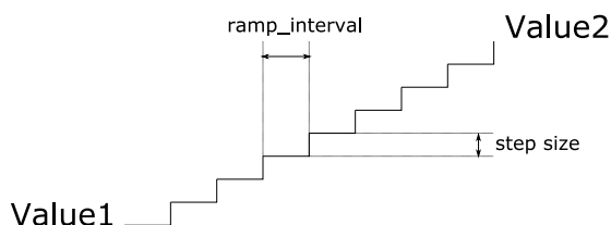
Figure 17. Ramping principle
