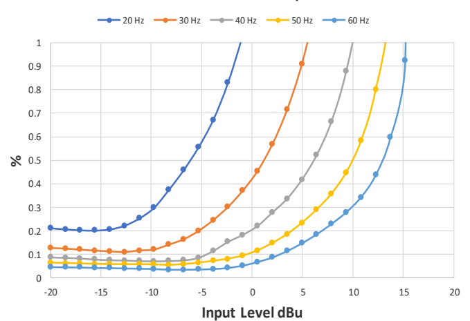
A-11J THD+N% at Fixed Frequencies
