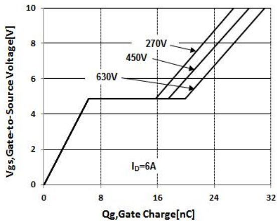
Figure 5. Gate-Charge Characteristics
