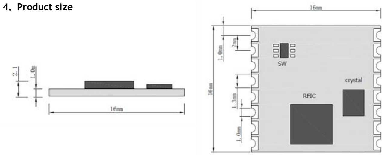
Figure 1: Module size
